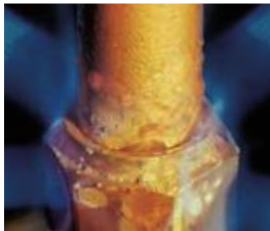
The flux becomes clear and watery as it approaches brazing temperature
